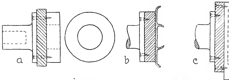
FIG. 318. BACKING FOR FACE-PLATE WORK.
